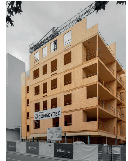
Wood integrated into urban residential buildings – 50 cross-laminated timber housing units built in Sabadell (Spain) by Conscytec, a subsidiary of Eiffage Energía in Spain
